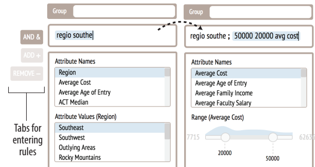
Figure 1: A user is entering sloppy rules to specify a group of colleges where \text{Region}=\text{Southeast} AND 20000 \leq \text{Average Cost} \leq 50000 . The sloppy rule menu has AND, ADD, and REMOVE tabs for entering base, inclusion, and exclusion rules respectively.
