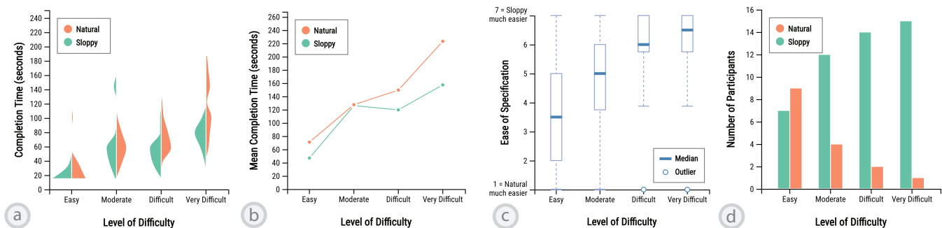
Figure 4: (a) Distributions of completion time at different difficulty levels. (b) Mean completion times for each interface at different difficulty levels. (c) Results of the Likert-scale question (Q1 of the questionnaire). (d) Participants' preference at each difficulty level (Q2 of the questionnaire).
