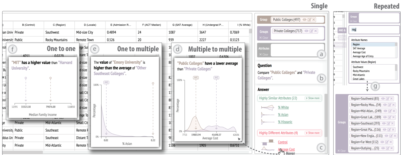
Figure 2: (a) Duo has three shelves for specifying pairwise comparison rules, and (b) displays the comparisons being performed in text. (c) For comparisons with the form “compare A to B”, it computes the similar and different attributes between the two groups. (d–f) When users hover over an attribute, the distributions are visualized. (g) When users partially specify an attribute but not a value using the sloppy rule menu, multiples groups are created to facilitate repeated pairwise comparison.
